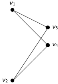
Figure 2: V = (G, E)
